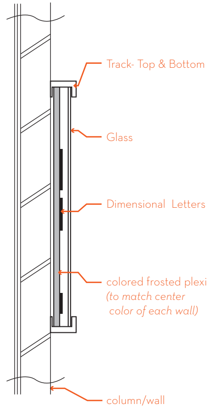
SECTIONAL VIEW
